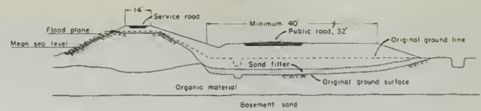
TYPICAL SECTION OF MASTER LEEVE
